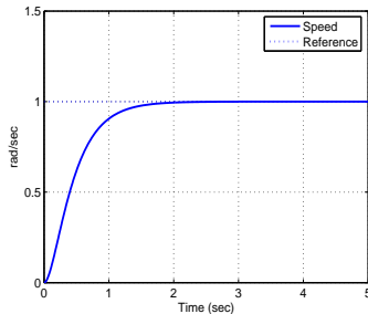
Fig. 3. Closed loop step response
