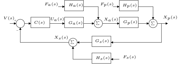
Fig. 1. Closed loop control with nonparametric faults
