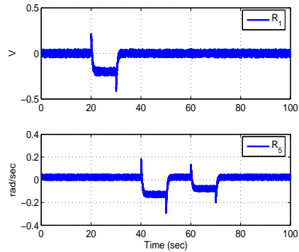
Fig. 4. Residuals R_1 and R_5
