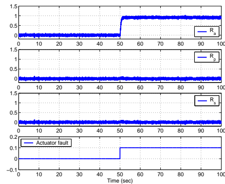
Fig. 7. Residual evolutions for changes in G_{\bar{a}}
