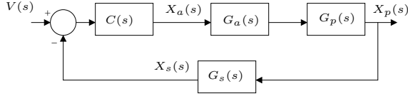
Fig. 2. Control loop with faulty components scheme
