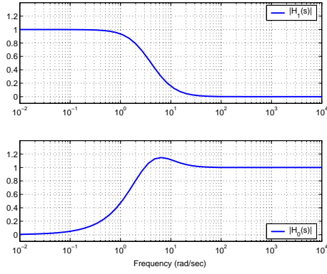
Fig. 5. Residual sensitivities
