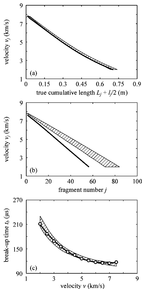
FIG. 8. Model fragmentation predictions. Barred area: experimental range, analytical modeling: ● Discrete values, — Mean curve.
