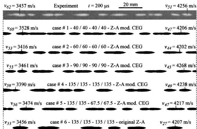
FIG. 2. Comparison of fragment geometry in experiment/simulations at 200 \mu\text{s} .
