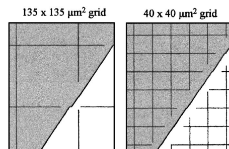
FIG. 6. Geometrical imperfections on the oblique surface of the liner for two different grids, at same location and same time ( 20 \mu\text{s} ).
