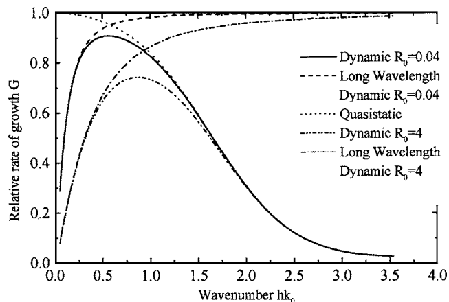
FIG. 9. Dispersion curves at initial time; influence of inertia ( \sigma_0=0, m=0.05 ). For the sake of clarity, the athermal stress is ignored in this figure. For consistency the strain rate sensitivity coefficient m is given a smaller value than in the rest of the paper.
