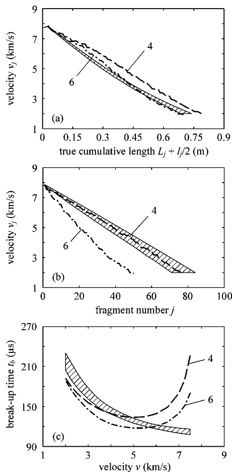
FIG. 3. Influence of model material on fragmentation predictions. Barred area: experimental range, simulation 4: Z-A mod. CEG, simulation 6: Z-A (see Table I).
