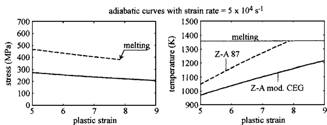
FIG. 1. Comparison of model materials used in numerical simulations. Initial state is taken in numerical simulations at 35 \mu\text{s} in an element at 5 \text{ km/s} : Simulation 6 with Z-A 87 model: initial strain=5, initial temperature = 1048 \text{ K} , Simulation 4 with Z-A mod. CEG model: initial strain=5, initial temperature= 970 \text{ K} .
