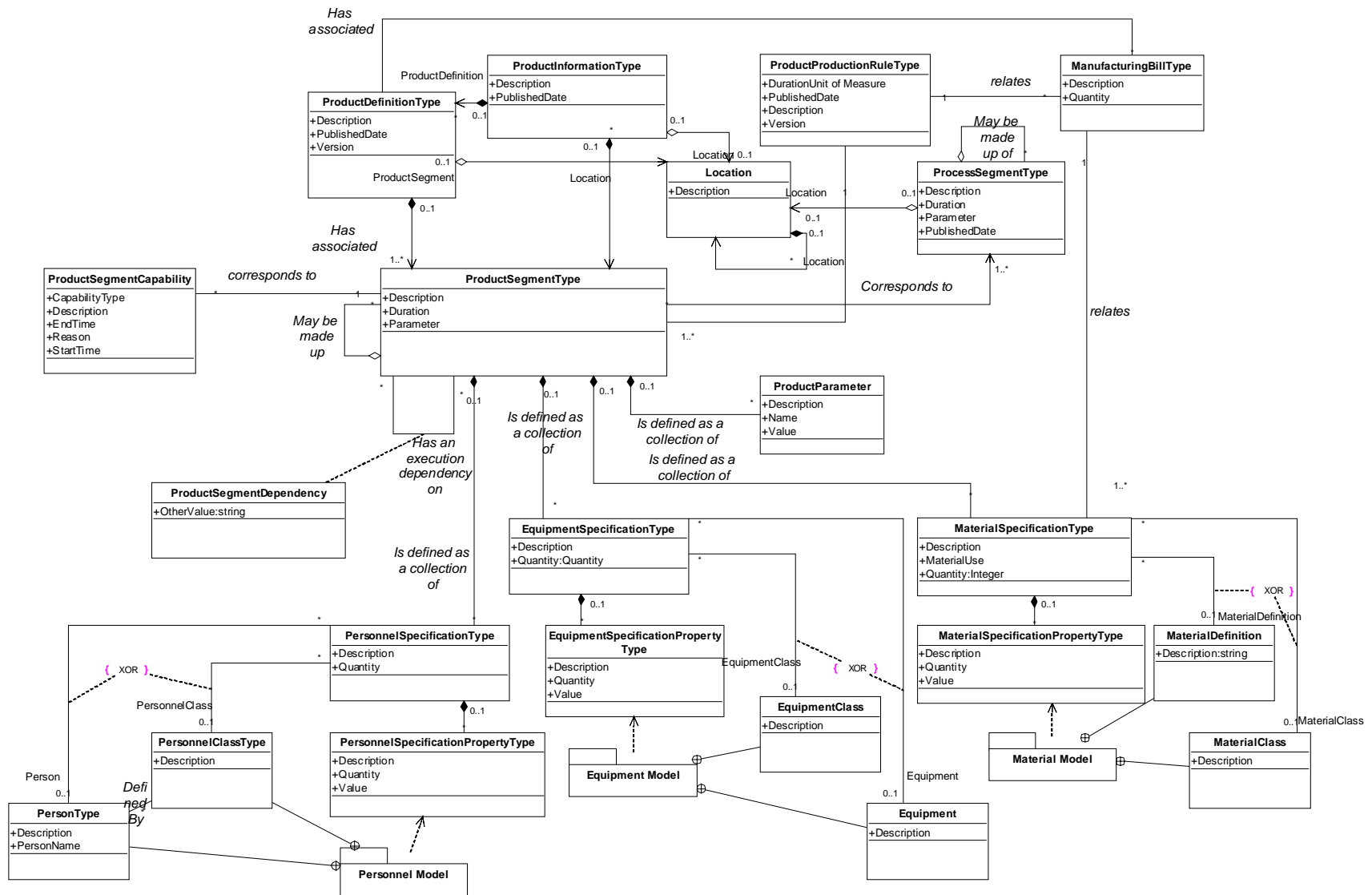
Figure 5: The conceptualised IEC 62264 Product Definition model
