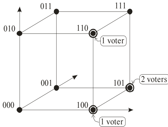
Figure 1 Geometric Representation of Ballots in 4-Voter Example (Voted-for Ballots Circled)
