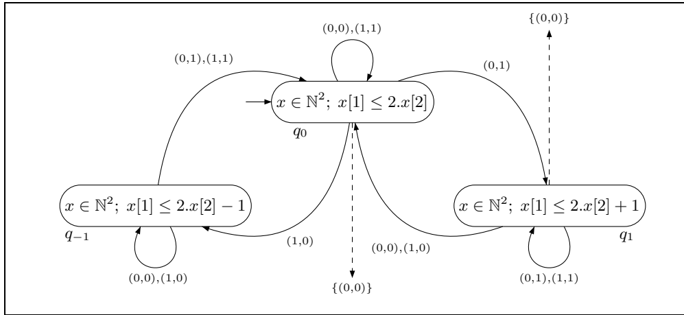
Fig. 14.4. The minimal FDVA \mathcal{A}_{2,2}(\{x \in \mathbb{N}^2; x[1] \leq 2.x[2]\})
