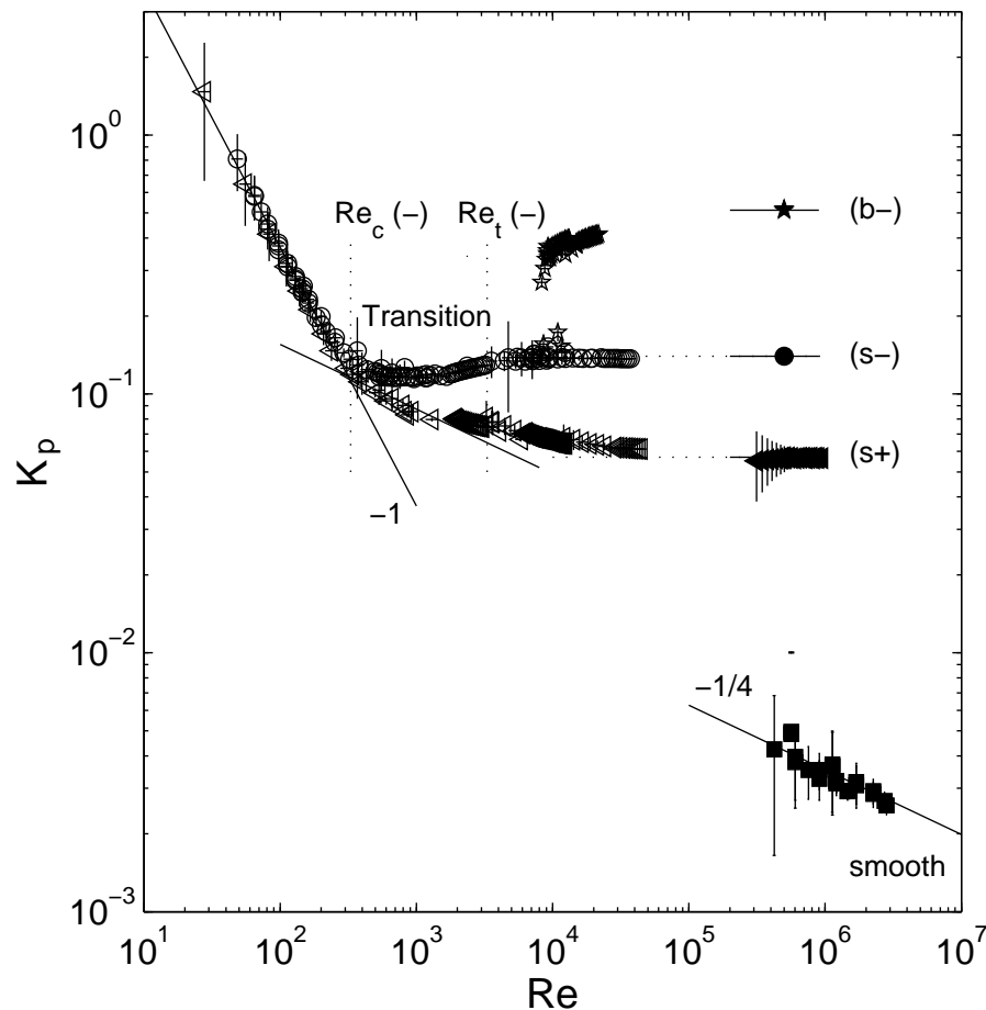
FIG. 9 Compilation of the dimensionless torque K_p vs. Re for various flows. All data stands for \mathcal{R}_\pi -symmetric von-Kármán flows except the branch labelled (b-) ( \star ): see caption of figure 7 for details. ( \circ ): direction of rotation (-). ( \triangleleft ): direction of rotation (+); the solid line is a non-linear fit of equation K_p = 36.9 \times Re^{-1} between Re = 30 and Re = 250 . Some data for flat disks of standard machine shop roughness, operated in pure water up to 25Hz (squares) are also displayed with a Re^{-1/4} fit. Another -1/4 power law is fitted for the positive direction of rotation for 330 \leq Re \leq 1500 and is displayed between Re = 10^2 and Re = 10^4 . Relative error on Re is \pm 10\% ; absolute error of \pm 0.1 N.m on the torque. Re_c and Re_t are the transition values computed from the fits of figure 5.
