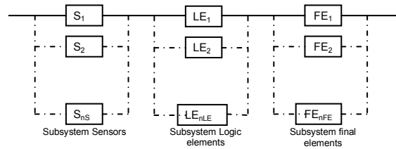
Fig. 4. Safety Instrumented System.
