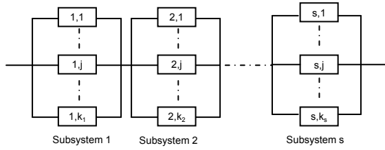
Fig. 1. General structure of parallel-series system.
