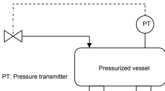
Fig. 3. Process diagram of example.
