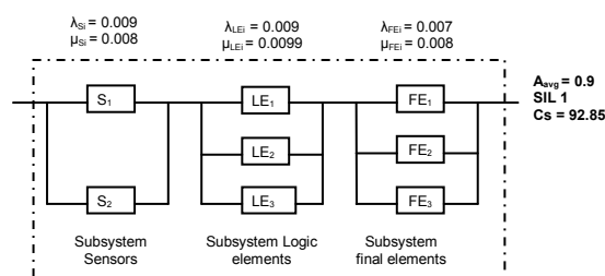
Fig. 6. Optimal SIS configuration.
