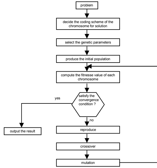
Fig. 2. A simple genetic algorithm framework.
