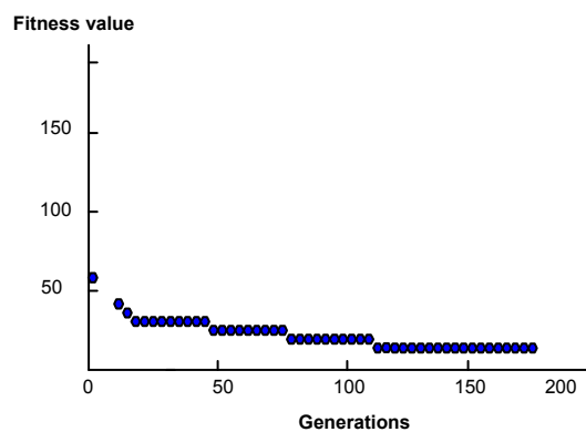
Fig. 5. Convergence results.
