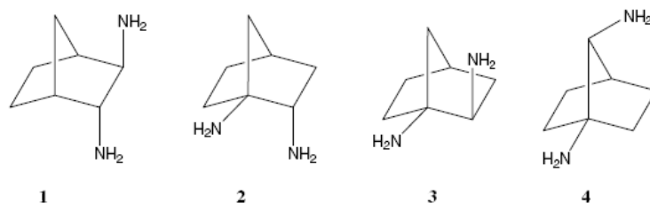
Scheme 2. Different norbornane-based 1,2-diamines envisaged.
