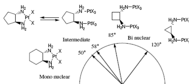
Scheme 1. Relationship between ligand bite angle and behaviour.
