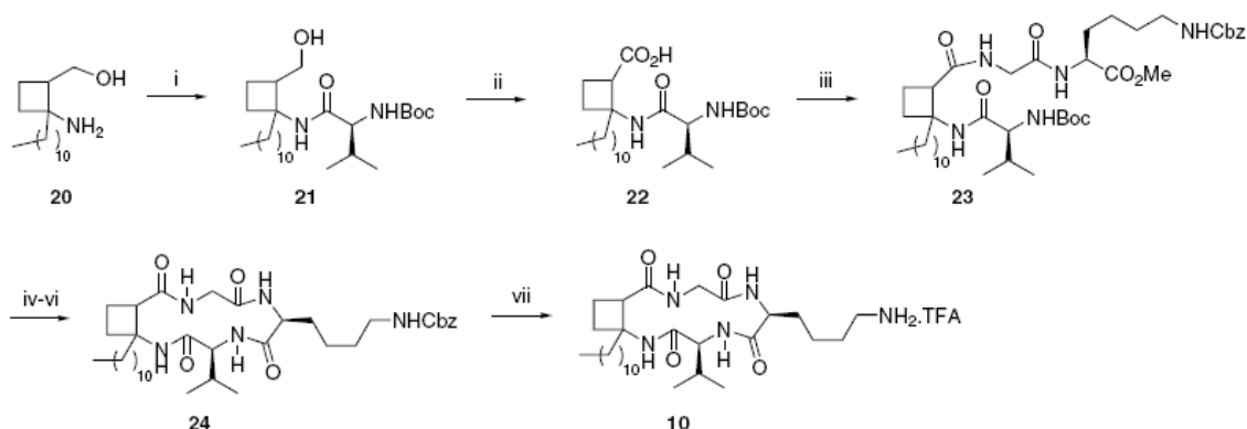
Scheme 4. Reagents and conditions: (i) Boc-Val-OH, EDC, HOBT, CH 2 Cl 2 , rt, 61%; (ii) cat. RuCl 3 , NaIO 4 , CCl 4 /CH 3 CN/H 2 O; (iii) H-Gly-N c -Cbz-Lys-OMe:TFA salt, Et 3 N, EDC, HOBT, CH 2 Cl 2 , rt, 31% (2 steps); (iv) LiOH, H 2 O/THF/CH 3 OH, 0 °C, then rt, 99%; (v) TFA, CH 2 Cl 2 , 0 °C, then rt, 98%; (vi) DPPA, NaHCO 3 , DMF, 5 °C, then rt, 71%; (vii) Pd/C 10%, TFA, CH 2 Cl 2 , 100%.
