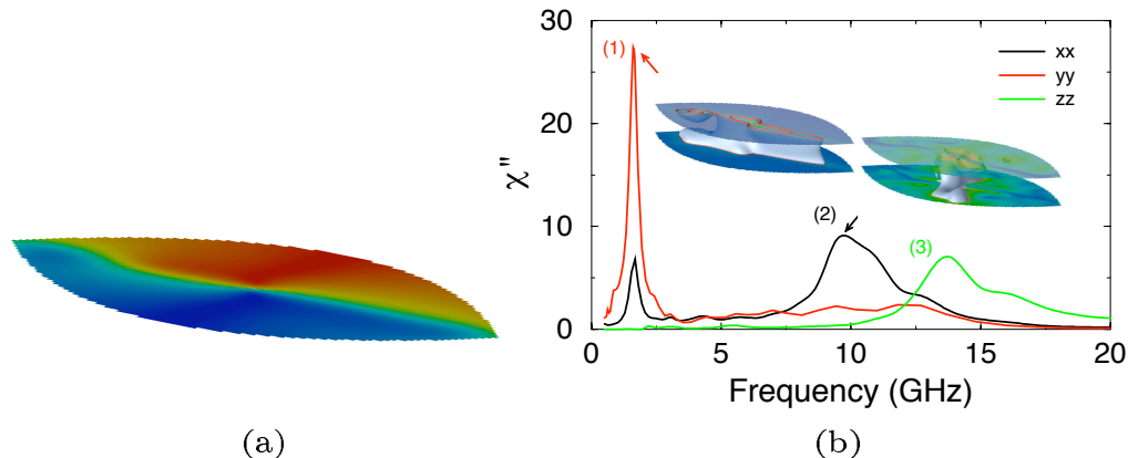
FIGURE 3. 3D micromagnetic simulations for an eye shape particle of sizes 320 \text{ nm} \times 640 \text{ nm} \times 80 \text{ nm} along the x , y and z axes, respectively. (a) Static magnetization component M_y at the bottom surface (positive values in red and negative values in blue). (b) Dynamic susceptibility spectra (imaginary part of the diagonal elements) with the spatial distribution of resonant modes in the color insets (high level in red and low level in blue).
