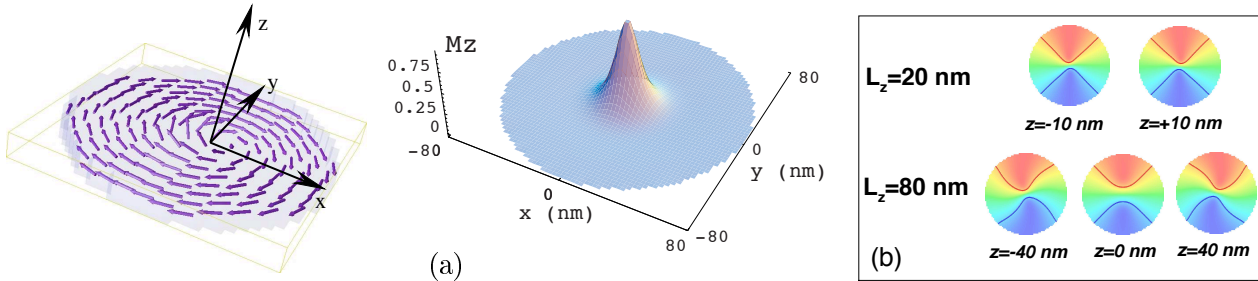
FIGURE 1. 3D static micromagnetic simulations for nanodots with radius R = 80 \text{ nm} supporting a vortex magnetic structure at the remanent state. (a) Representation of the vortex-like structure and coordinate system. (b) M_x maps for two thicknesses L_z = 20 \text{ nm} and L_z = 80 \text{ nm} . The color maps correspond to views in the (x, y) plane at different z positions (high level in red and low level in blue).
