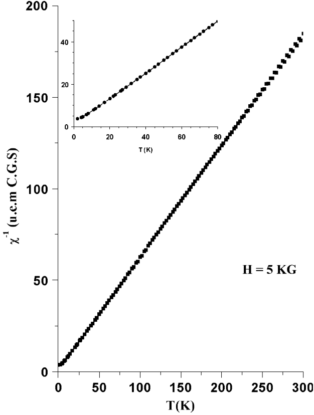
Fig. 8. Reciprocal molar magnetic susceptibility of \text{Fe}_{0.50}\text{TiO}(\text{PO}_4) as a function of temperature.
