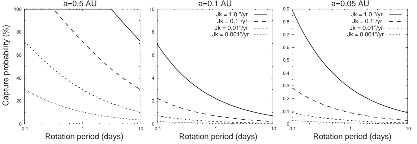
Fig. 2. Obliquity capture probabilities in resonance ( \nu_k = -10.0 ''/yr) under the effect of gravitational tides, as a function of the rotation period at a) 0.5 AU b) 0.1 AU c) 0.05 AU. J_k is the amplitude of secular orbital perturbations (see. Eq.8). Physical parameters are taken from HD 209458b.
