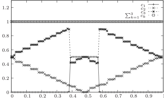
Modified limited downwind scheme.
