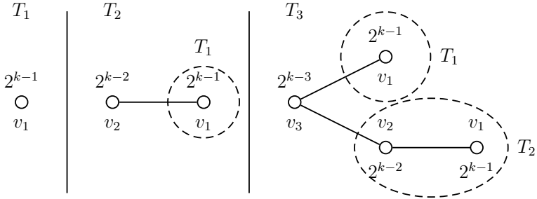
Figure 4: Gadgets for T_1, T_2 and T_3 .
