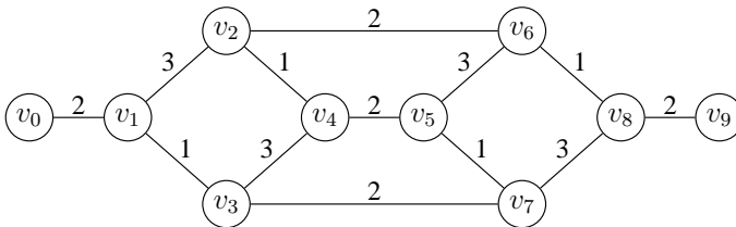
Figure 7: Gadget F_2 for e \in E_2 .
