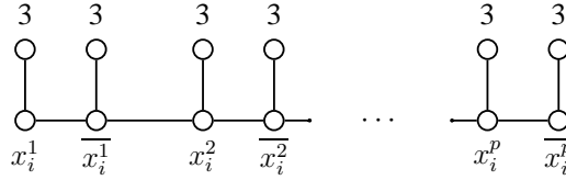
Figure 3: Graph H(x_i) representing variable x_i
