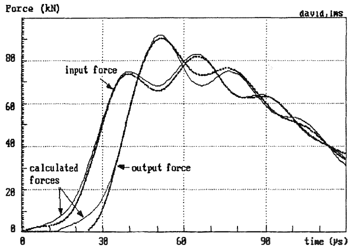
Fig. 3 Comparison between simulated and measured forces (SHPB)
