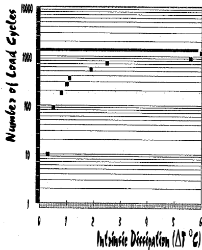
Fig. 4 Fatigue lifetime evaluation of a column base of the reinforced concrete structure subjected to seismic type loading.
