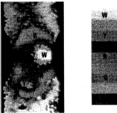
Fig. 1 Infrared thermography of a concrete specimen under vibratory compressive excitation: weakness zones are readily detected by heat patterns after 7,000 load cycles (0.2 °C for each color hue).
