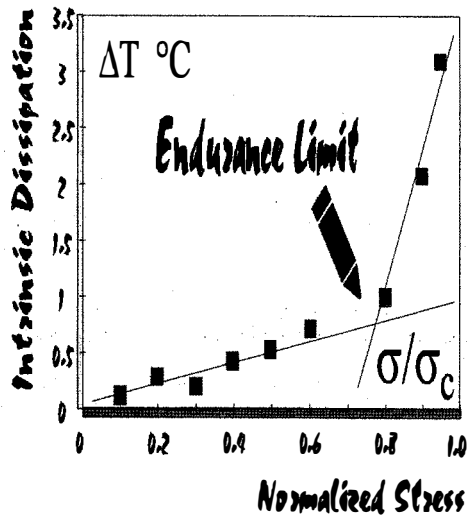
Fig. 2 Graphical determination of the fatigue limit of a concrete specimen.
