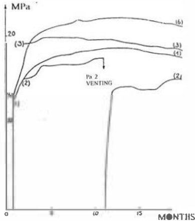
Figure 8 - Pressure build-up in closed caverns at Vauvret (Pa1, Pa2, Pa3, Pa6).
