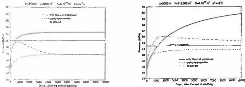
Figure 5 - Pressure build-up in a small, shallow cavern (a) or a large, deep cavern (b).
