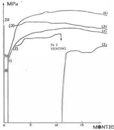
Figure 8 - Pressure build-up in closed caverns at Vauvret (Pa1, Pa2, Pa3, Pa6).
