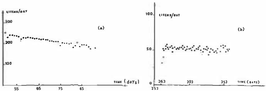
Figure 3 - Brine flow expelled from open cavern EZ53 [Hugot, 1988].
