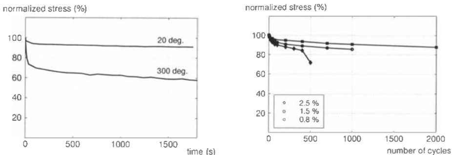
Figure 1. Experimental observations on aluminum alloy : (a) exponential shape of relaxation in TRC tests, (b) negligible cyclic softening behavior in LCF tests
