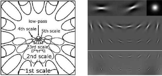
Fig. 19. Multiresolution scheme with 6 orientations and 5 scales. (Left) Schematic contours of the filters in the Fourier domain. The Fourier domain origin (DC component) is located at the center of the inset and the highest frequencies lie on the border. (Right) Real (symmetric) part of the filters in the space domain. Scales are arranged in rows and orientations in columns. The two first scales are drawn at the bottom magnified by a factor of 4 for a better visualization. The low-pass filter is drawn in the upper-right part.
