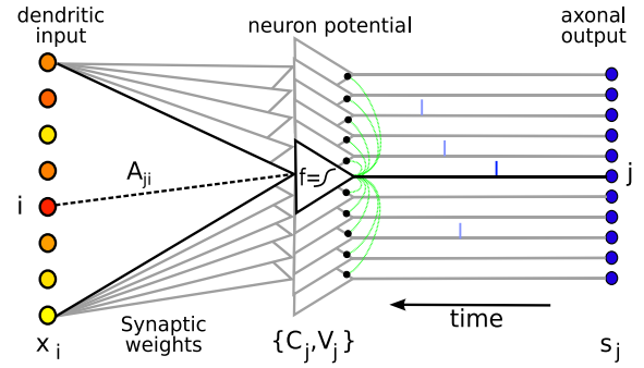
Fig. 15. Model of a neuronal layer as a communication channel. To understand the content of neural activity, we consider here that the neuronal layer implements the inverse of a forward model (that is the analysis in Fig. 12). The architecture is similar to the perceptron: the input (noted x_i ) is matched with normalized weight patterns A_{ji} (which are fixed in this section) so as to provide an integrative activation value (the membrane potential) which in turn is non-linearly transformed to achieve a membrane potential which grows proportionally to the probability of matching a feature. Spikes represent decisions that are fed back on the correlated neighboring neurons using lateral interactions (that we represented for the first spiking neuron) but also on the axonal output which yield a spiking output s_j .
