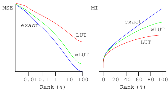
Fig. 8. Progressive reconstruction of the image from the spike list using rank-order coding. We plotted ( Left ) the Mean-Squared Error (MSE, logarithmic scale on the abscissa) and ( Right ) the Mutual Information (MI) using the different temporal spike codes described in the text. We compared the results of the propagation when knowing the coefficients (exact) with the method described in Eq. 21 (LUT) which uses an optimized Look-Up-Table to "guess" the value of the coefficients from their rank. Finally we compared these strategies to the optimized method that uses the regularity found in natural images through the statistics of natural images (wLUT). The reconstruction from this latter method is close to the method with exact values and proves that the analog values may be transmitted using rank order coding. It therefore constitutes a compact spike code which provides a simple implementation of rank-order coding for static images.
