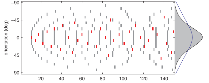
Fig. 16. Implementation of the greedy pursuit using Integrate-and-Fire Neurons. We simulated here the activity of a network of Integrate-and-Fire neurons tuned to form a simple model of an hyper-column in the primary visual area (V1) to the presentation of a horizontal edge at t = 0 . We show in this image the output spiking activity of 16 neurons tuned for different orientations for the feed-forward (black bars) and the sparse spike coding (white bars) models during the first 150 ms. In this latter model, the correlation linked to the information already detected is propagated as a hyper-polarizing and shunting lateral interaction to the neighboring neurons: the response in both latency and spiking frequency to the oriented edge is clearly more selective. (Right Inset) Output spike firing rate to the presentation of a horizontal edge at time t = 0 . For the linear feed-forward model (plain line), the sparse spike coding scheme (filled curve) for different orientations of the input stimulus. The narrower tuning curve for the latter method represents a more selective response to the features learned in synaptic weights and mimics the behavior of the neural response in the primary visual area [Ringach, 2002].
