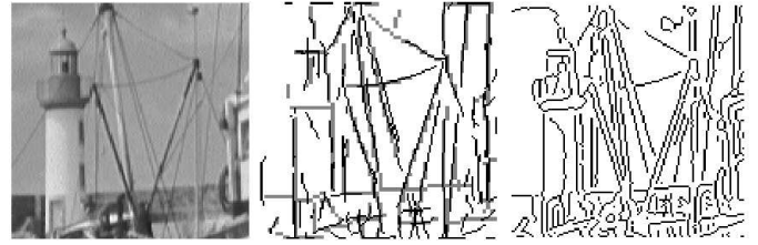
Fig. 22. Edge extraction using the multi-scale representation. (Left) 128×128 pixel image "Boats". (Middle) Edges extracted by sparse Gabor wavelets. 1st scale and 2nd scale edges appear in black. The 3rd scale edges appear in gray, they are plotted larger since the 3rd scale is downsampled and offers coarser spatial localization. (Right) Edges extracted by Canny method [Canny, 1986; Deriche, 1987]. The SEC method extracts edges which are subjectively more accurate. Reconstruction of the image using these edges revealed qualitatively better results (see [Fischer et al., 2006b]).
