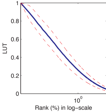
Fig. 20. Regularity of edge coefficients distribution in natural images. We plotted for 200 natural images the mean and variance (depicted by the dotted lines representing the mean \pm one standard deviation) of the decrease of coefficients values in the probabilistic Matching Pursuit scheme described above as a function of the rank. Assuming that these values represent the edge content of the images, it shows that the probability distribution of edge coefficients is regular in natural images and may be used in an efficient compression scheme. It permits to evaluate the coefficients quickly as a function of the rank, and since the transmission error being proportional to the variance to transform efficiently an analog image in a wave of spikes. It should be noted that this decrease is much more rapid than the one observed in the model retina the coefficients are below .15 after 1% of relative rank (to compare with Fig. 7).
