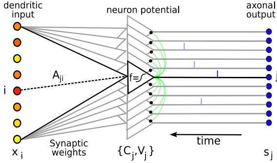
Fig. 15. Model of a neuronal layer as a communication channel.
