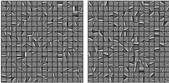
Fig. 17. Results using the sparse-hebbian learning scheme with 196 filters. Starting with random filters, we compared here the results of the learning schemes using ( Left ) the classical conjugate gradient function ('cgf') method as is used in [Olshausen and Field, 1998] with ( Right ) the Sparse Spike Coding method. Results replicate the original results of [Olshausen and Field, 1998] and are similar for both methods: both dictionary consist at convergence of Gabor-like filters which are similar to the receptive fields of simple cells in the primary visual cortex [Ringach, 2002]. Edges appear in these conditions to be the independent components of natural images. However, it should be noted that the Sparse Spike Coding method introduces less localized filters and a higher proportion of high-frequency Gabors when no efficient homeostatic rule was defined [Perrinet, 2004a, 2006]. All scripts generating figures and control experiments are available, see Sec. 3.4.3)
