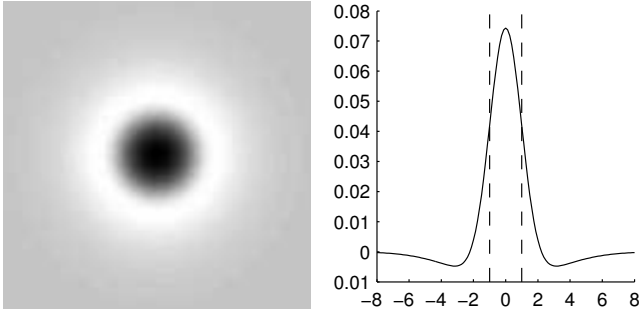
Fig. 5. Mother function for the filters in the retina. (Left) The DOG filter is a center-OFF (in black) surround-ON (in white) contrast detector. (Right) Central profile of the DOG filter. As a unit measure, the vertical striped lines represent the variance of the narrower Gaussian used to generate the DOG filter and thus corresponds to the center of neighboring filters.
