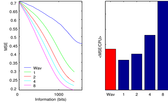
Fig. 13. Is the spike representation over-complete in the retina? (Left) We compared the progressive transmission of information for different degrees of over-completeness in the retina by plotting the average MSE of the residual as a function of the information to code the spike list (in logarithmic scale, propagation up to 12.5% of the relative rank for clarity). The set of neurons used rotation symmetric Mexican hat filters, with scales from layer to layer growing as \rho = \{2, \sqrt{2}, \sqrt[4]{2}, \sqrt[8]{2}\} (and denoted on the legend respectively as 1, 2, 4 and 8). As a comparison we plotted the method used in [van Rullen and Thorpe, 2001] (line 'Wav'). As a function of rank, the MSE decreases more rapidly for increasing degrees of over-completeness. (Right) But if we plot the trade-off of MSE with CPU usage as a function of the over-completeness, we find that for the same amount of information the adaptive dyadic strategy is optimal. One should note that the results of the method described in the text is better than the wavelet method of [van Rullen and Thorpe, 2001] since it is adaptive.
