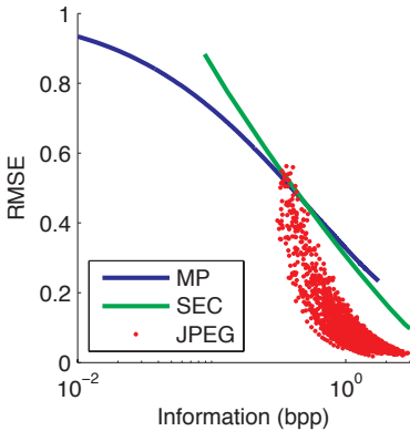
Fig. 21. Compression efficiency of MP compared to SEC and JPEG. We compared the coding efficiency measured as the normalized root mean squared error (RMSE) as a function of the coding entropy (in bytes per pixel). A RMSE of 0 means a perfect reconstruction, while a RMSE of 1 means that the error is maximum (null image). Three phases corresponding to the three method appear in the graph. The MP method is capable of coding with very low entropy starting at relatively low efficiency, but getting progressively better. The JPEG method is not adapted to low-entropy coding but gets very good results after a medium quality parameter (around 60 and 1 bpp). The SEC method gives intermediate results of good efficiency in rather low entropy ranges.
