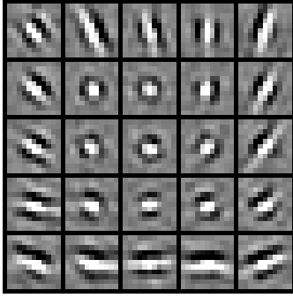
Fig. 26. Emergence of a topological set of orientation selective filters. As presented above, we simulated the emergence of filters in the primary visual area but introduced lateral connections between filters so that neighboring spiking filters (and thus learning filters) was enhanced. This led to the emergence of topological relations between neighboring filters similar to the neuro-physiologically observed pinwheels : all different orientations are present while preserving a smooth transition between neighboring filters. Note that the center gets less selective (since the constraint is higher than in the periphery), an observation which is contested in physiology.
