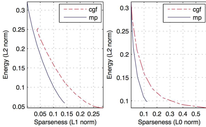
Fig. 14. Efficiency of the matching pursuit compared to conjugate gradient. We compared here the matching pursuit ('mp') method with the classical conjugate gradient function ('cgf') method as is used in [Olshausen and Field, 1998]. We present the results for the coding of a set of image patches drawn from a database of natural images. These results were obtained with the same fixed dictionary of edges for both methods. We plot the mean final residual error for two definitions of sparseness: (Left) the mean absolute sum of the coefficients and (Right) the number of active (or non-zero) coefficients (the coding step for MP). For this architecture, the sparse spike coding scheme appears to be more efficient to code natural image patches.
