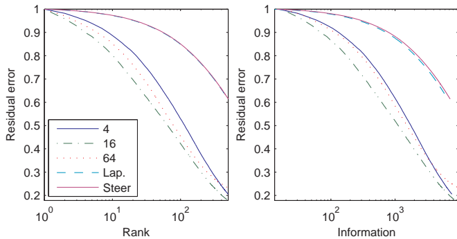
Fig. 25. Efficiency of the Sparselet Analysis. We compared here the sparselet analysis scheme at different levels of over-completeness with classical methods. We plot the residual Mean Squared Error (MSE) over a set of 1000 natural images for different numbers of spikes. (Left) The MSE is plotted in function of this number : the sparse spike coding algorithm outperforms the laplacian (Lap.) and steerable pyramid (Steer.) linear representations and gets better as the over-completeness increases. (Right) When plotting the MSE as a function of an approximate of the information needed to code the spike list, the increase of efficiency is less marked: these strategies have similar efficiency.
