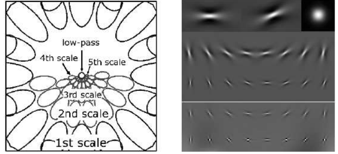
Fig. 19. Multiresolution scheme with 6 orientations and 5 scales. (Left) Schematic contours of the filters in the Fourier domain. The Fourier domain origin (DC component) is located at the center of the inset and the highest frequencies lie on the border. (Right) Real (symmetric) part of the filters in the space domain. Scales are arranged in rows and orientations in columns. The two first scales are drawn at the bottom magnified by a factor of 4 for a better visualization. The low-pass filter is drawn in the upper-right part.
