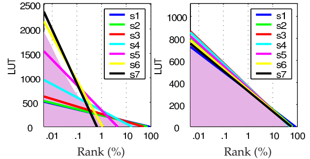
Fig. 7. Optimization of the regularity of the wavelet coefficients with harmonized scales. (Left) The LUT (Eq. 21) is shown in the background in plain color as a function of the relative rank (in %) using a logarithmic scale on the abscissa. When separating the LUT for the different scales (from lowest to highest : s_1 to s_7 in the legend), one may observe that they correspond to similar regularities —linked to the regular distribution of singularities at different scales— but are mistuned (lower frequencies, as the 7 th scale ‘ s_7 ’ are stronger and thus decrease more rapidly as a function of the overall rank). These regularities are therefore lost and mixed when ranking all scales together. (Right) By normalizing the different scales according to the statistics of natural images, the “vote” by the ranking process becomes “fair” and the LUTs for the different scales better match. The resulting LUT for harmonized scales preserves the underlying regularity and information transmission is therefore more robust (see Eq. 25): it represents a more effective way to encode the analog value by the rank of a spike.
