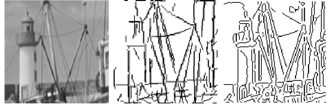
Fig. 22. Edge extraction using the multi-scale representation. (Left) 128 \times 128 pixel image "Boats". (Middle) Edges extracted by sparse Gabor wavelets. 1st scale and 2nd scale edges appear in black. The 3rd scale edges appear in gray, they are plotted larger since the 3rd scale is downsampled and offers coarser spatial localization. (Right) Edges extracted by Canny method [Canny, 1986; Deriche, 1987]. The SEC method extracts edges which are subjectively more accurate. Reconstruction of the image using these edges revealed qualitatively better results (see [Fischer et al., 2006b]).
