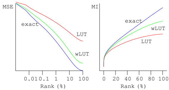
Fig. 8. Progressive reconstruction of the image from the spike list using rank-order coding. We plotted ( Left ) the Mean-Squared Error (MSE, logarithmic scale on the abscissa) and ( Right ) the Mutual Information (MI) using the different temporal spike codes described in the text. We compared the results of the propagation when knowing the coefficients (exact) with the method described in Eq. 21 (LUT) which uses an optimized Look-Up-Table to “guess” the value of the coefficients from their rank. Finally we compared these strategies to the optimized method that uses the regularity found in natural images through the statistics of natural images (wLUT). The reconstruction from this latter method is close to the method with exact values and proves that the analog values may be transmitted using rank order coding. It therefore constitutes a compact spike code which provides a simple implementation of rank-order coding for static images.
