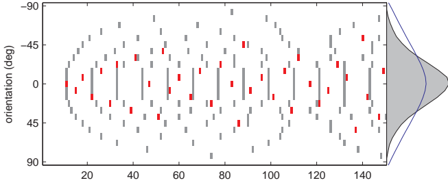
Fig. 16. Implementation of the greedy pursuit using Integrate-and-Fire Neurons. We simulated here the activity of a network of Integrate-and-Fire neurons tuned to form a simple model of an hyper-column in the primary visual area (V1) to the presentation of a horizontal edge at t = 0 . We show in this image the output spiking activity of 16 neurons tuned for different orientations for the feed-forward (black bars) and the sparse spike coding (white bars) models during the first 150 ms. In this latter model, the correlation linked to the information already detected is propagated as a hyper-polarizing and shunting lateral interaction to the neighboring neurons: the response in both latency and spiking frequency to the oriented edge is clearly more selective. (Right Inset) Output spike firing rate to the presentation of a horizontal edge at time t = 0 . For the linear feed-forward model (plain line), the sparse spike coding scheme (filled curve) for different orientations of the input stimulus. The narrower tuning curve for the latter method represents a more selective response to the features learned in synaptic weights and mimics the behavior of the neural response in the primary visual area [Ringach, 2002].
