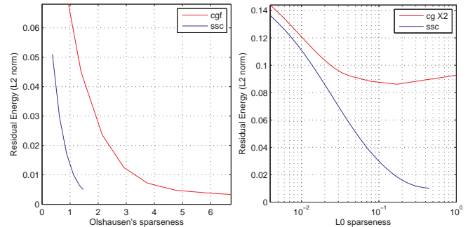
Fig. 18. Efficiency of the matching pursuit compared to conjugate gradient. We compared here the matching pursuit ('ssc') method with the classical conjugate gradient function ('cgf') method as is used in [Olshausen and Field, 1998] for the coding of a set of 10000 image patches drawn from a database of natural images. We plot the mean final residual error and the signal to noise ratio (in dB) as a function of two definitions of sparseness : ( Left ) the mean absolute sum of the coefficients (the sparseness defined in [Olshausen and Field, 1998]) and ( Right ) the number of active (or non-zero) coefficients (the coding step for MP) which provides an estimate of the coding efficiency (in bits) for the image patch. The conjugate gradient function approach was applied twice ('cg X2', see text). For this architecture, the sparse spike coding scheme proves to be more efficient to learn and code natural image patches. The approximate solution for the hard constraint (Eq. 29) is therefore more efficient on both constraints costs.
