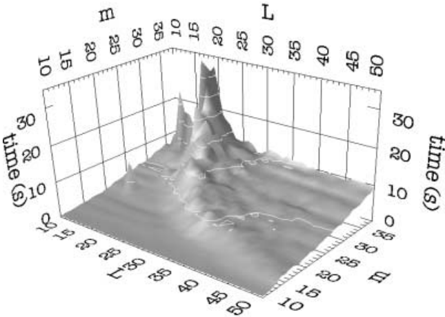
Fig. 2. \theta -subsumption cost(m, L) for MCS, averaged on 1,000 pairs (C, Ex) m : nb predicates in C in [10,38] , L nb constants in Ex in [10,50] (scale factor \times 6 compared to Fig. 1)
