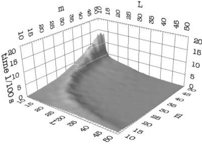
Fig. 3. \theta -subsumption cost( m, L ) for Django.V8 , averaged on 1,000 pairs (C, Ex) (scale factor \div 25 compared to Fig. 1)
