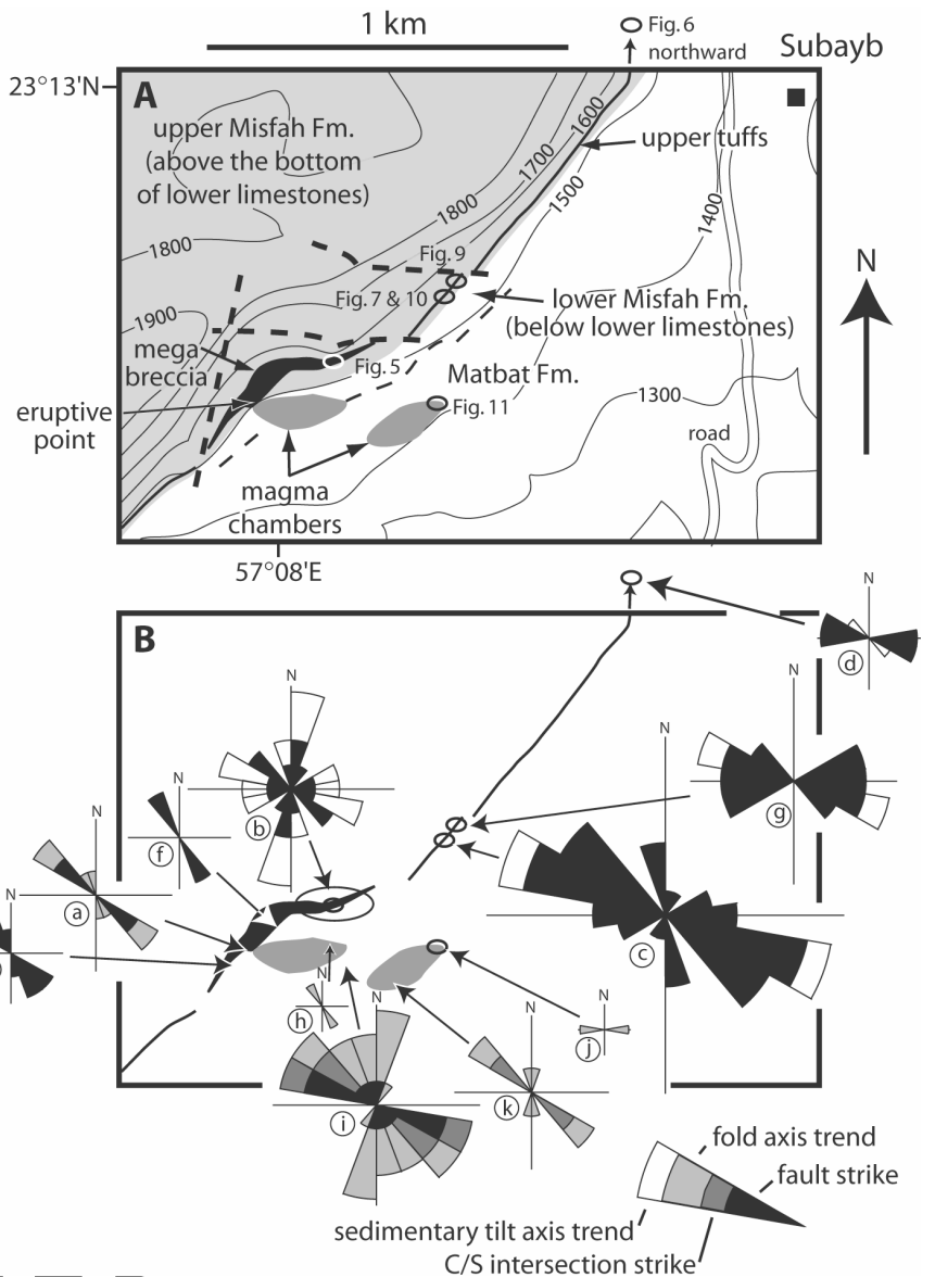
Figure 3: (A) Schematic geological map of the studied area. Topography (meters) from Beurrier et al., 1986 . Thick stippled lines are recent faults, thin stippled line represents the unobserved limit between Misfah and Matbat formations. Figures 5 to 7 and 9 to 11 are located by ellipses. (B) Same as Figure 3A, with location of the upper tuffs, megabreccia and magma chambers and rose diagrams of structural observations. Rose diagrams (a) to (k), see comments in the text. Same scale for all rose diagrams, maximum seven values on rose c. All structural measurements are related to the same magmatic event, with the exception of N-S structures at sites (i) and (k) which are related to a more recent eastward normal shear.
