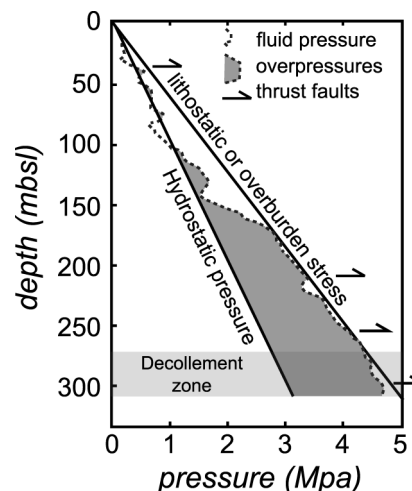
Figure 2. Pressure profile for pore fluid at the toe of the Barbados wedge (modified after Moore and Tobin [1997]).
