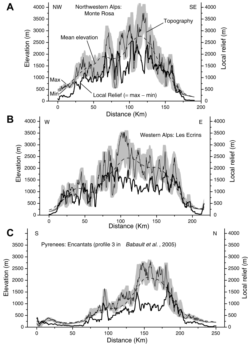
Figure 1. Relationship between mean elevation and local relief in the western Alps and the Pyrenees. (a) Northwest to southeast ( 7^{\circ}1'46''54' ; 8^{\circ}23'45''29' ) topographic profile across the northwestern Alps. (b) West to east ( 4^{\circ}57'44''57' ; 7^{\circ}43'45''02' ) topographic profile across the western Alps. (c) South to north topographic profile across the Central Pyrenees. The three profiles have been performed using the same method [see Babault et al. , 2005]. Note that along the profiles across the Alps a decrease in the local relief can be observed in some places where the mean elevation is high, indeed possibly due to the occurrence of glaciers, but none of these profiles shows the particular pattern observed in the Pyrenees, precluding a glacial origin for the high-elevation, low-relief surfaces seen in the Central Pyrenees.
