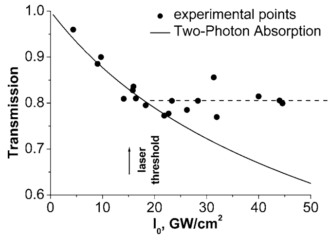
FIG. 2. Experimental and theoretical nonlinear transmission curves at 700 \text{ nm} . The arrow indicates lasing threshold.
