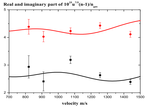
FIG. 4: Plot of the real (squares) and imaginary (dots) parts of 10^{25}u^{7/5}(n-1)/n_{gas} measured for xenon as a function of the lithium beam mean velocity u ( n_{gas} in \text{m}^{-3} , u in m/s). The full curves represent the calculated values [15], using the Buckingham-Corner potential of ref. [19]. The agreement between the measured and calculated values is good, especially as there are no free parameters.
