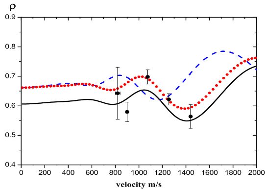
FIG. 5: Plot of the ratio \rho = \text{Re}(n-1)/\text{Im}(n-1) for xenon as a function of the lithium beam mean velocity u . The points are our experimental values while the curves have been calculated with the lithium-xenon potential of references [19] (full line), [22] (dotted line) and [23] (dashed line).
