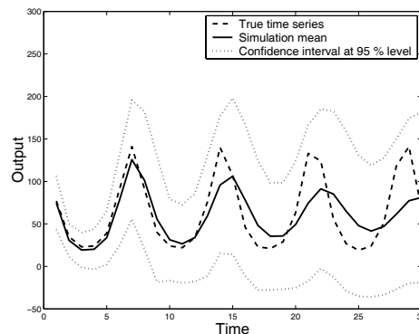
Figure 6. Comparison for the first 30 values between the mean of the 1000 simulations (solid) and the true values of the test set (dashed), together with confidence intervals at 95% level (dotted).
