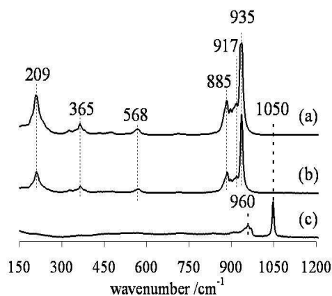
Fig. 2 : Raman spectra of (a) precipitate from a NiMo solution (b) NiMo 6 H 6 O 24 (NH 4 ) 3 Anderson solid and (c) the NiMo filtered solution
