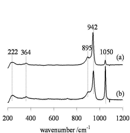
Fig. 1 : Raman spectra before precipitation of (a) CoMo solution and (b) NiMo solution
