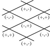
Figure 8: Signature changes.
