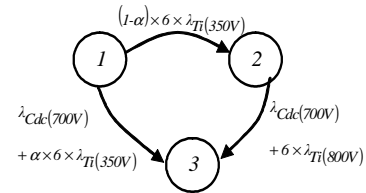
Fig. 10. Markov Chain for modelling the system with four legs shunt S_2 .
