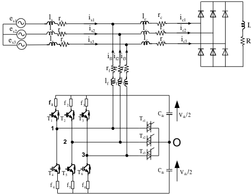
Fig.2: Fault tolerant three-legs shunt active filter: S_1 .
