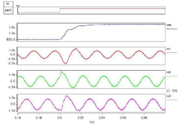
Fig. 6. Current and voltages dynamic behaviour for \mathcal{S}_1
