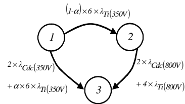
Fig. 9. Markov Chain for modelling the system with three legs shunt S_1 .
