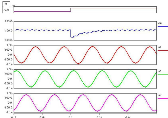
Fig. 7. Current and voltages dynamic behaviour for S_2
