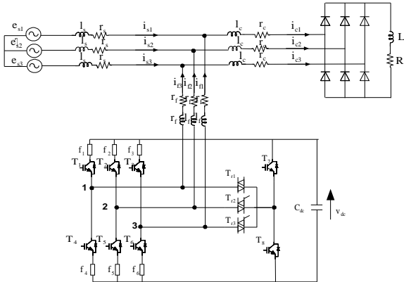
Fig.3: Fault tolerant four-legs shunt active filter: S_2 .
