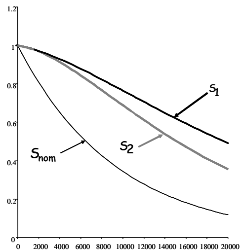
Fig. 11. Reliability computation.
