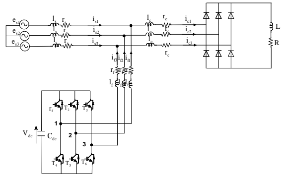
Fig.1: Classical three-leg shunt active filter: S_{nom} .
