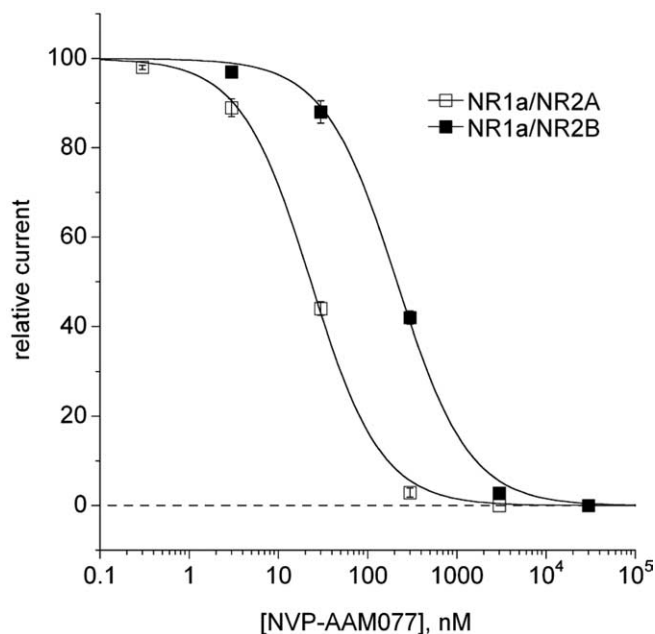
Figure 1. NVP-AAM077 discriminates poorly between NR2A- and NR2B-containing receptors. Concentration–response curves showing NVP-AAM077 inhibition of rodent NR1a/NR2A and NR1a/NR2B receptors expressed in Xenopus oocytes, as described by Perin-Dureau et al. (2002), are shown. NMDAR currents were elicited at -60 mV using glycine at a saturating concentration ( 100 \mu\text{M} ) and glutamate at a concentration close to EC_{50} ( 5 \mu\text{M} for NR1a/NR2A and 2 \mu\text{M} for NR1a/NR2B receptors). NVP-AAM077 was applied during an application of glutamate plus glycine. The inhibition was quantified once the response in NVP-AAM077 had reached steady state. The curves represent least-square fits to the data points using the following equation: I_{rel} = 100 - 100 / (1 + (IC_{50} / [NVP-AAM077])^n) . The estimated values of IC_{50} and n values are: 23 nM and 1.10 for NR1a/NR2A receptors and 213 nM and 1.07 for NR1a/NR2B receptors. Each point is the mean value obtained from five to eight cells. NVP-AAM077 stock solutions ( 1 mM and 100 \mu\text{M} ) were prepared by progressive dilutions with bidistilled water of a solution containing 10 mM NVP-AAM077 in 100 mM NaCl. Error bars represent SD.
