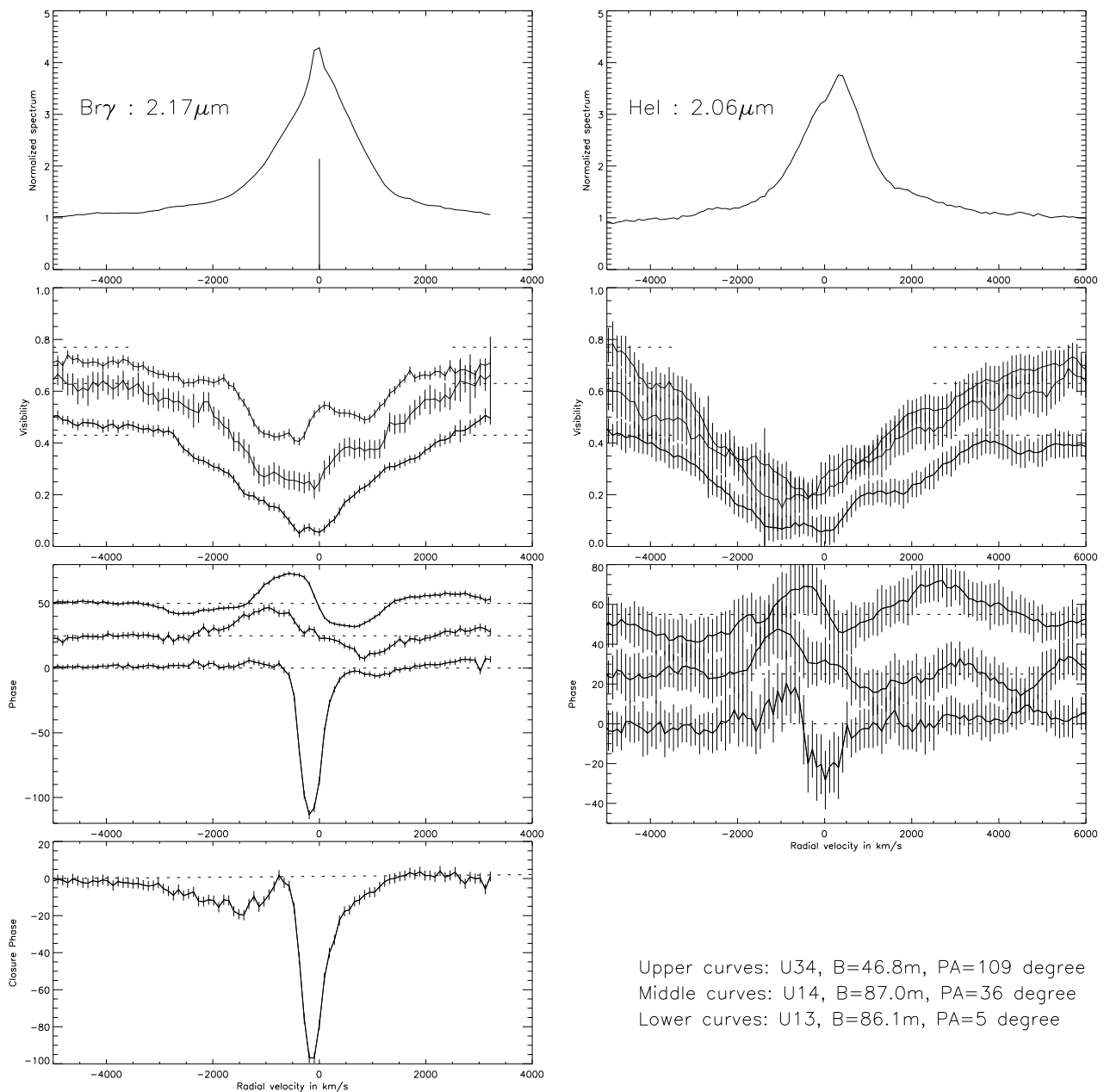
Fig. 2. AMBER observables extracted from the data recorded the 2006 February 18: 1) AMBER spectrum of the Br \gamma (left) and HeI (right) lines. 2) Visibilities for the three baseline (upper line U34, middle U14, lower U13). The mean continuum levels of the high SNR data (dotted lines) are overplotted for comparison. 3) Differential phases (upper line U34, middle U14, lower U13). The U14 and U13 lines are shifted by 25 and 50 degrees, respectively. The mean continuum levels (dotted lines, zero level) are overplotted for comparison. 4) The closure phase. The dotted line emphases the zero level. All the curves result from the interpolation of the measurements by straight lines.
