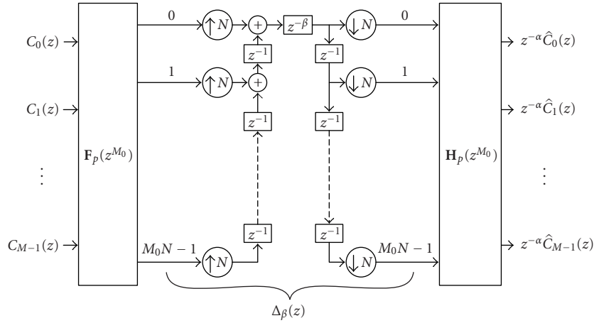
FIGURE 2: BFDM/QAM transmultiplexer with a simplified polyphase implementation.
