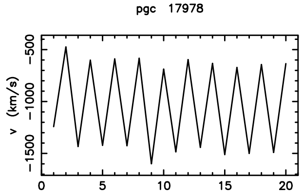
Fig. 7. The evolution of peculiar velocities with respect to the number of iterative loop. Here are the two first galaxies in our sample, and an exceptionally “bad” case (pgc 17978) which was rejected from the final analysis.
