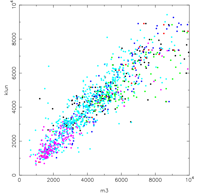
Fig. 10. Comparison of MarkIII and KLUN distances expressed in \text{km.s}^{-1} . The colors represent the different Mark III samples (Willick et al. 1997): HMCL is black, W91CL red, W91PP green, CF blue, MAT turquoise, and A82 purple.
