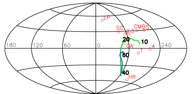
Fig. 13. Upper panel shows the amplitude of the observed bulk motion within a growing sphere of radius R_{\text{max}} , and the corresponding \Lambda CDM expected curve for a flat cosmological model using : n = 1 , \Omega_b = 0.04 , h = 0.57 , and \Omega_m = 0.22 \pm 0.02 . The bottom panel show the direction of the bulk flow, in galactic coordinates, and its evolution with R_{\text{max}} = 10\text{--}60h^{-1} Mpc. The main published results as listed in Table 6 are also shown.
