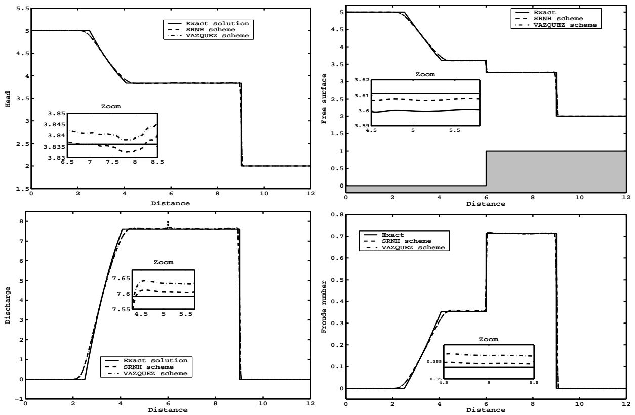
Figure 4.3: Subcritical flow past a forward facing step at time t = 0.5 s.
