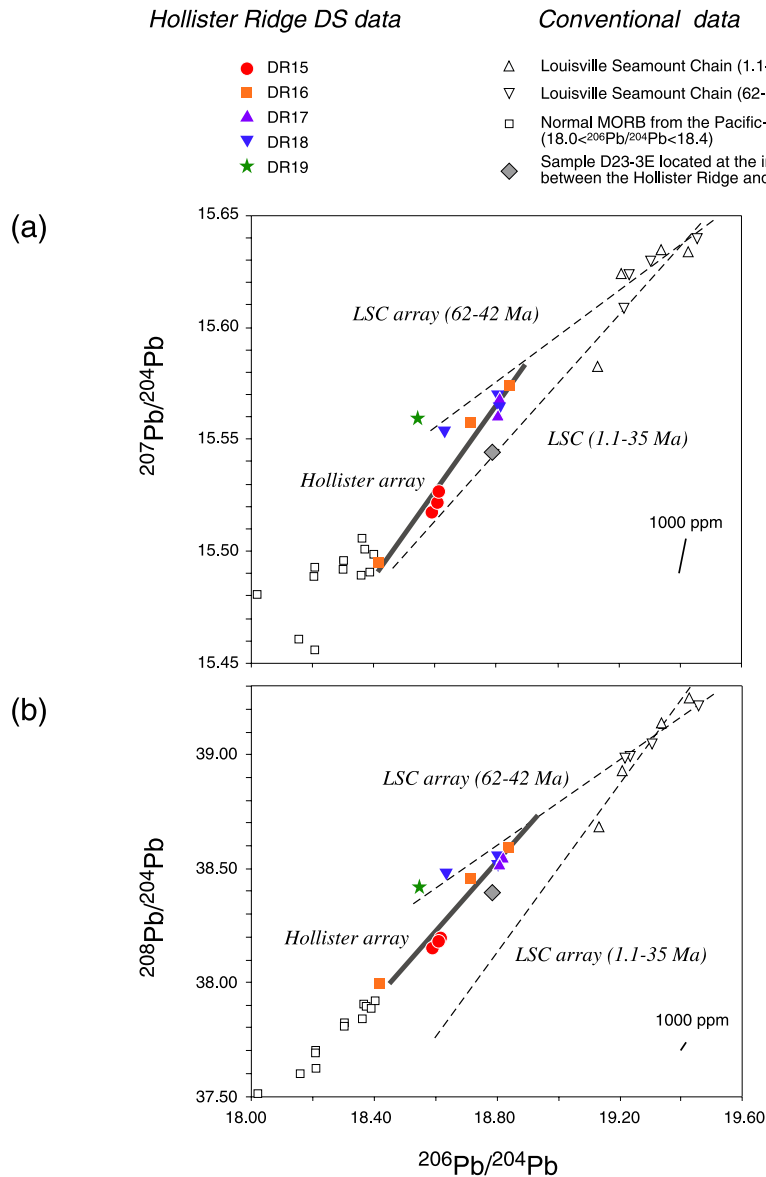
Figure 4. Comparison between the isotopic signature of Hollister Ridge and those of the Louisville Seamount Chain and the Pacific-Antarctic Ridge. Literature data [Cheng et al. , 1987; Castillo et al. , 1998; Vlastélic et al. , 2000] have been renormalized to the NBS981 values obtained with the SBL74 double spike (see Table 1), as explained in the Figure 2 caption. The error bars shown (1000 ppm) are the typical external error ( 2\sigma ) of conventional data. Double spike data are about ten times more precise [Dosso et al. , 2002].
