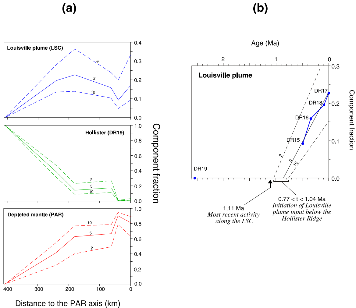
Figure 5. Three end-component mixing model. The three mantle components involved are (1) the Hollister component, the composition of which is best represented by sample DR19 (see Table 1); (2) the Louisville plume component, the composition of which ( ^{206}\text{Pb}/^{204}\text{Pb} = 19.29 , ^{208}\text{Pb}/^{204}\text{Pb} = 39.032 ) is taken from Cheng et al. [1987]; and (3) the PAR component, the isotopic composition of which ( ^{206}\text{Pb}/^{204}\text{Pb} = 18.256 , ^{208}\text{Pb}/^{204}\text{Pb} = 37.737 ) is that of unradiogenic MORB ( ^{206}\text{Pb}/^{204}\text{Pb} < 18.40 ) from south of the Udintsev fracture zone [ Vlastélič et al. , 2000]. The model does not require knowing the absolute concentration of Pb in the different mantle components. Only the relative Pb enrichment has to be considered. The two “enriched” components (Louisville and Hollister) are assumed to have the same Pb concentration. These sources are enriched relative to the depleted mantle by a factor that is not known precisely. Factors of 2, 5, and 10 (numbers indicated on the lines) are considered for the lower limit, best estimate, and upper limit, respectively. (a) Component fractions plotted against the distance to the PAR axis. (b) Louisville plume fraction plotted against the age of the lavas. For clarity, data points are shown only for an enrichment factor of 5. However, regression lines are shown for the different enrichment factors and used to estimate the age of the initiation of Louisville plume contribution to the Hollister Ridge source. (a, b) Averaged values are used for each dredge location.
