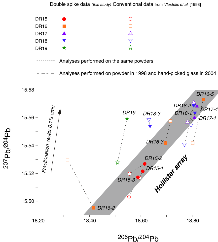
Figure 2. Comparison between double spike and conventional data. In order to show only the effect of precision, conventional data [from Vlastelic et al. , 1998] have been renormalized to the NBS981 values obtained with the SBL74 double spike (see Table 1) using a linear mass fractionation law: R_{cor} = R_{conv}(1 + \epsilon\delta m) , where R_{cor} and R_{conv} are the corrected and conventional isotopic ratios, \delta m is the mass difference between the two isotopes of the ratio, and \epsilon is the mass discrimination coefficient per mass unit. \epsilon is inferred from the same equation knowing the isotopic composition of the NBS981 each data set refers to. A mass fractionation plot vector of 0.1%/amu is shown. With the exceptions of samples DR18-3 and DR19, the new, highly precise data plot along a linear array (gray band).
