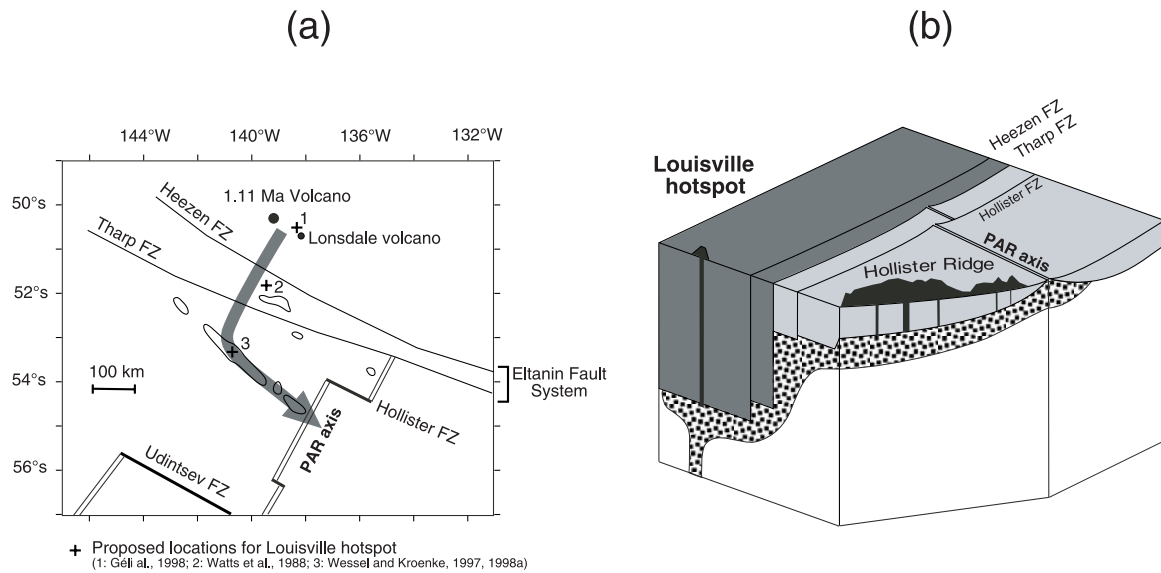
Figure 6. Louisville plume–Pacific-Antarctic Ridge interaction model. (a) Map showing the respective positions of the youngest volcanoes of the Louisville Seamount Chain (LSC), the Eltanin Fault System, Hollister Ridge, and the Pacific-Antarctic Ridge. The youngest seamount sampled along the LSC ( 50^{\circ}27'S – 139^{\circ}10'W ) is now dated at 1.11 \pm 0.04 Ma [Koppers et al., 2004]. Petrologic and isotopic data [Hawkins et al., 1987; Cheng et al., 1987] indicate unambiguously that this seamount originates from the Louisville hot spot. About 90 km southeast of the 139^{\circ}10'W seamount, at 50^{\circ}54'S – 138^{\circ}6'W , Lonsdale [1988] also mapped a volcano (named “Lonsdale volcano” in the map), which is also a candidate for the present site of the hot spot. Crosses indicate the location of the hot spot inferred from kinematic models. The location proposed by Géli et al. [1998], near “Lonsdale volcano,” reconciles both geochemical and kinematics constraints and is used in this study to model the plume-ridge interaction. Because the hot spot is located at a great distance (1300 km) from the opposite spreading segment (Heezen-Raitt) of the East Pacific Rise, but only 120 km north of the Heezen FZ, a limb of the plume (gray arrow) may be diverted southward, where the lithosphere is much younger and thinner. Then, the plume material is expected to flow toward the nearby spreading axis, as suggested in common plume-ridge interaction models. During this last step, the flow may have been captured by the preexisting lithospheric crack through which Hollister Ridge most likely emplaced [Géli et al., 1998]. This figure shows that Hollister Ridge lies along the shortest path of pressure release linking the Louisville hot spot to the Pacific-Antarctic ridge and explains why Hollister Ridge samples the plume-ridge flow. (b) Cartoon illustrating the shortest path of pressure release linking the Louisville hot spot to the Pacific-Antarctic ridge.
