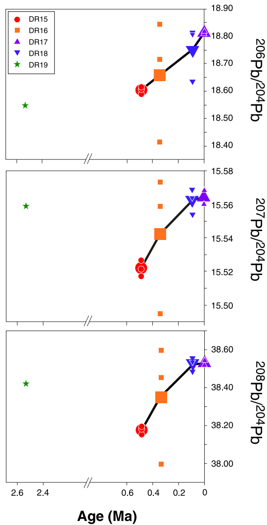
Figure 3. Pb isotope ratios plotted versus age. One sample per dredge was dated [Vlastélic et al. , 1998]. These ages are taken as representative of the dredges. Within dredge isotopic variation (DR16 and DR18) may reflect the sampling of distinct lava flows. The larger symbol represents the mean values of individual samples.
