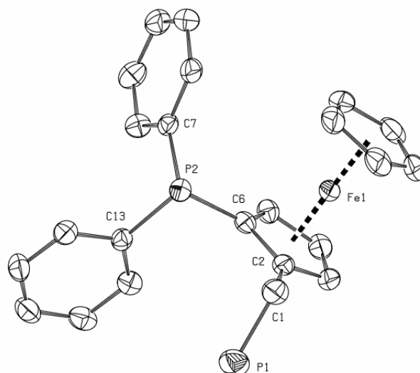
Fig. 1. ORTEP drawing of diphosphine 2 .
