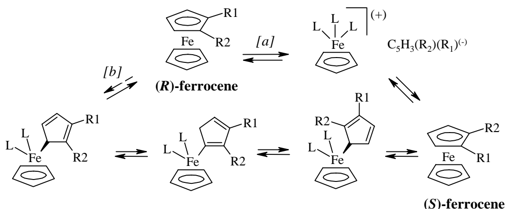
Scheme 6. Intramolecular racemisation processes for chiral ferrocenes.
