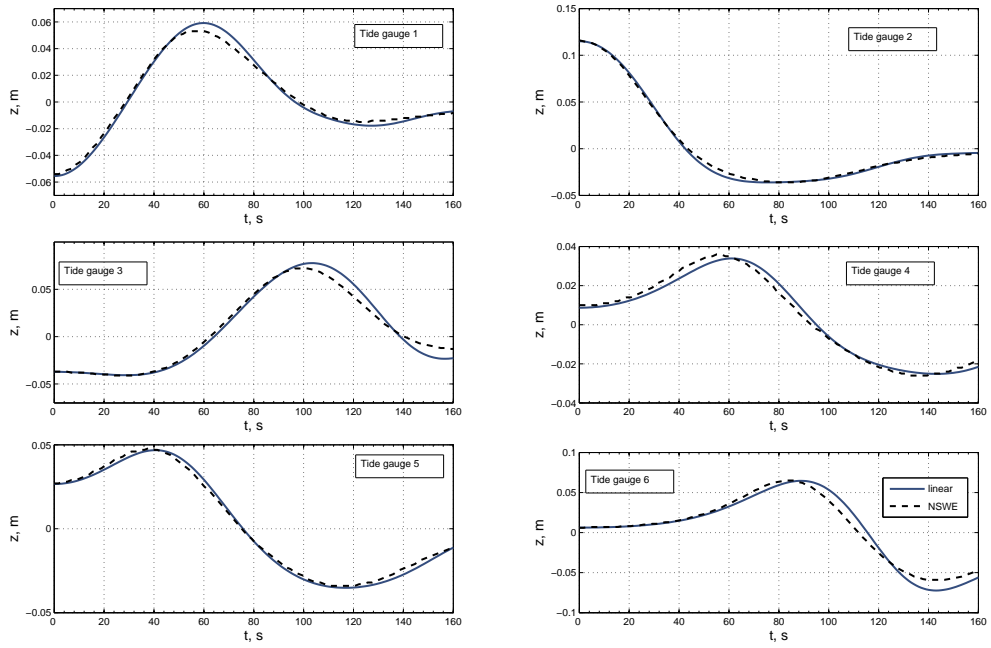
Figure 9: Transient waves generated by an underwater earthquake. Comparisons of the free-surface elevation as a function of time at the selected gauges shown in figure 8: —, linear model ; - - nonlinear shallow water model. The time t is expressed in seconds. The physical parameters are those of figure 7. Since the fully nonlinear results cannot be distinguished from the linear ones, they are not shown.
