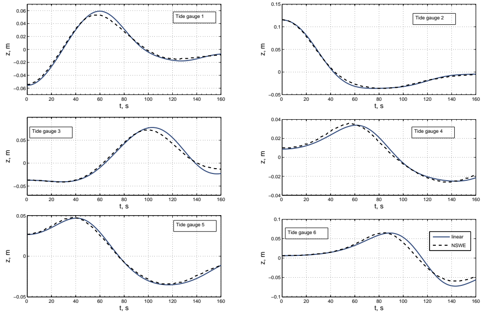
Figure 9: Transient waves generated by an underwater earthquake. Comparisons of the free-surface elevation as a function of time at the selected gauges shown in figure 8: —, linear model ; - - nonlinear shallow water model. The time t is expressed in seconds. The physical parameters are those of figure 7. Since the fully nonlinear results cannot be distinguished from the linear ones, they are not shown.
