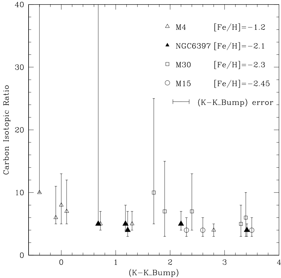
Fig. 1. Evolution of the carbon isotopic ratio with respect to the stellar K_s -magnitude above the bump in the RGB luminosity function of each globular cluster. The adopted K_s -bump magnitudes are reported in Table 1. The maximum error on (K_s - K_s^{\text{Bump}}) is shown in the upper right corner and, for a given cluster, the uncertainty on the relative stellar luminosities with respect to their bump is \pm 0.04 mag. (see text for more details). The reported metallicity (in dex) of each GC is from Kraft & Ivans (2003). For two stars (one in M4 and one in NGC 6397), we have only been able to derive upper limits for their carbon isotopic ratios. These limits are represented by a symbol located at the lower end of their error bar.
