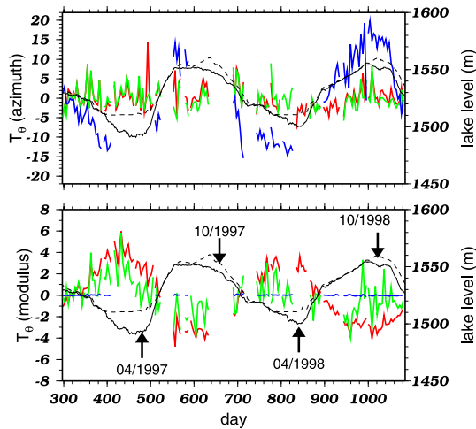
Figure 7. Observed real vector T_0 , (bottom) modulus and (top) azimuth versus time (day 297 = 23/10/1996) for 3 dipoles, LGB (red), VEW (green), and BBW (blue). Thin lines are for the Roselend (solid line) and La Gittaz (dashed line) lake levels. The average of modulus and azimuth have been removed for the dipole comparisons.
