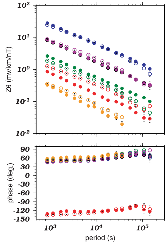
Figure 2. Amplitude and phase of Z_{\theta 1} (open symbols) and Z_{\theta 2} (solid symbols) for 5 of the dipoles. Red, BBE; green, BRC; blue, CNE; purple, EWS; orange, BBW (Figure 1).
