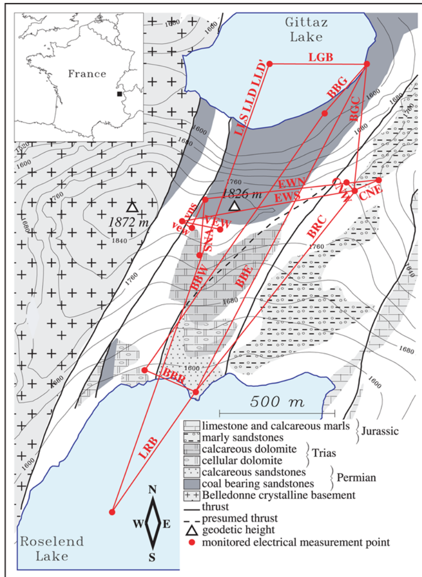
Figure 1. Geological map of the Sur-Frètes area, showing the location of the electrical measurement points and the dipole array.
