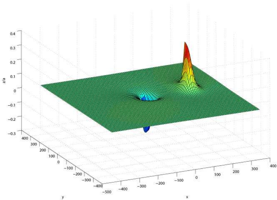
FIGURE 4. Dimensionless free-surface deformation z/a after strike-slip fault. Here a is |\mathbf{D}| (30 m in the present application).
