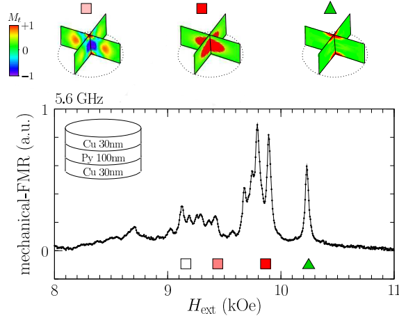
FIG. 3: Mechanical-FMR spectrum of a single t = 100 nm thick Py layer disk ( \phi = 1 \mu\text{m} ) at 5.6GHz. The lowest energy mode is interpreted as a mode localized at the surface of the disk, shown as a triangle. Squares denote the uniform and magnetostatic modes. The top shows the transverse dynamics of the main modes represented in a color code, calculated using a micromagnetic simulation.
