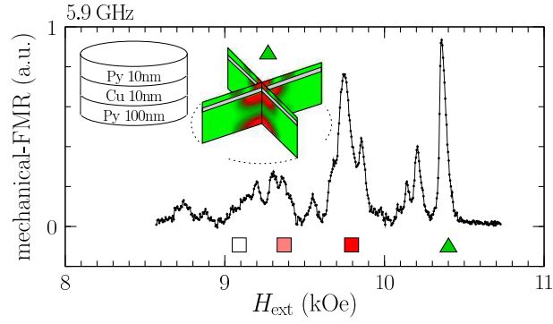
FIG. 4: Mechanical-FMR spectrum of a double layer Py disk ( \phi = 1 \mu\text{m} ) with thicknesses of 10 nm and 100 nm at 5.9 GHz. The spacer is a 10 nm thick Cu layer. The lowest energy mode is associated to a coupled precession between the localized mode of the thick layer and the dynamics of the thin layer. The inset is a result of a micromagnetic simulation.
