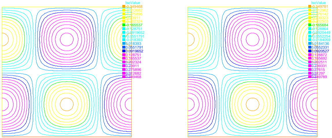
FIGURE 4. These two figures show respectively the exact and numerical pressure's solutions.
