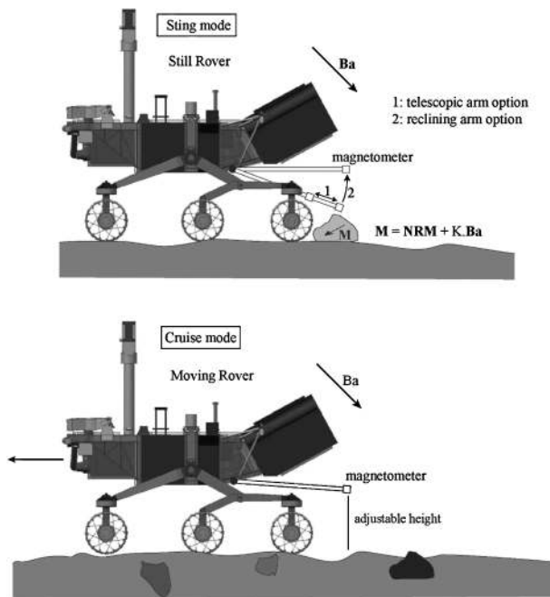
FIG. 1. Sketch of the MSL rover with the proposed placement of the MAREDD instrument at the end of a deployable boom. K , magnetic susceptibility; M , magnetization.
