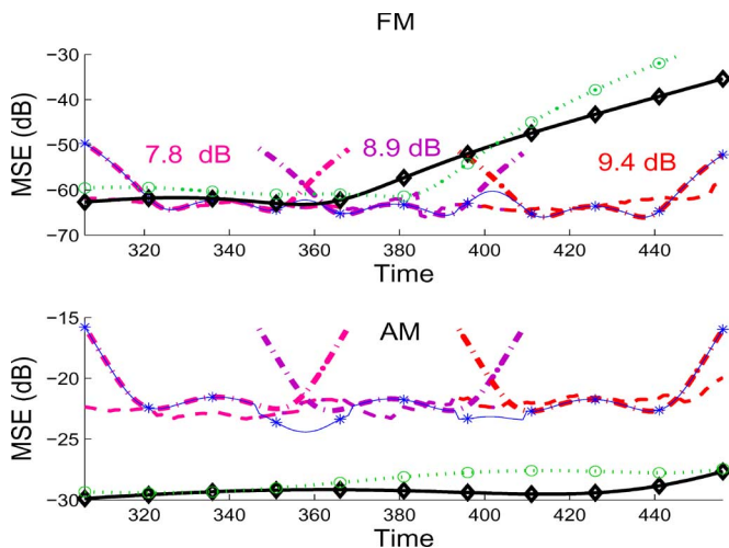
Fig. 9. Zoom in the right column of Fig. 8 (SNR = 7 dB): (---) MSE and (- · -) \text{CRB}_I for each segment, ( \diamond ) \text{CRB}_P calculated for the true orders, ( \circ ) \text{CRB}_P calculated for FM order = 9 and AM order = 4, and ( \ast ) \text{CRB}_G derived after segmentation and smoothing strategies.
