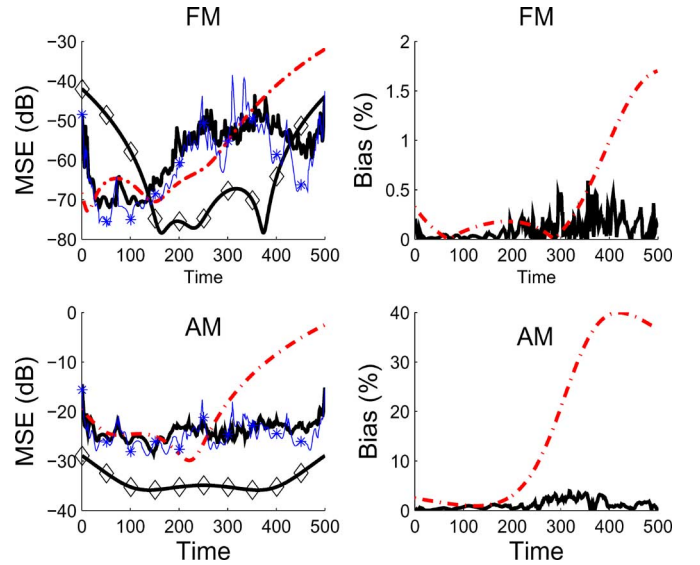
Fig. 5. MSE of the IA and IF estimates of the signal of (23) at a mean SNR = 15 dB: (---) HAF-based method, (—) the proposed method, (—◇—) the \text{CRB}_P , and (—×—) the \text{CRB}_G .
