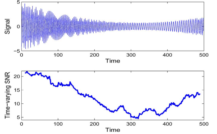
Fig. 4. Noisy signal of (23) and the time-varying SNR (decibels) which is computed by using a sliding window of 20 samples.
