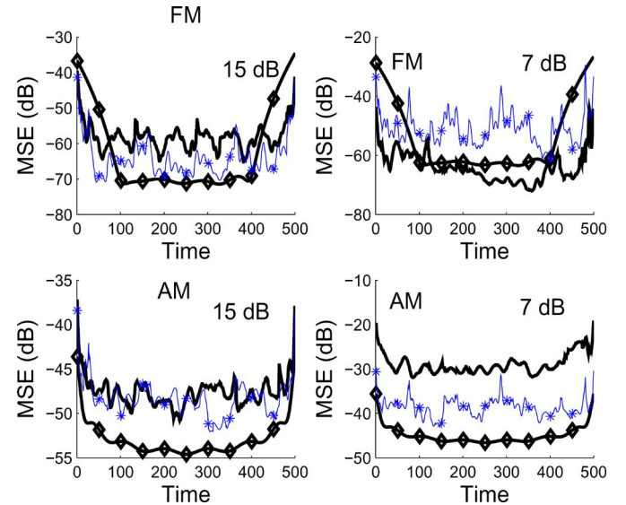
Fig. 11. MSE (---) of the sinusoidal AM and FM estimates. The \text{CRB}_P are calculated at a mean SNR = 15 dB (left column) and SNR = 7 dB (right column) for a polynomial approximation of the seventh-order for both AM and FM.
