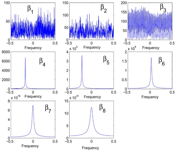
Fig. 7. HAF transform of the signal in Fig. 1 as calculated for the phase coefficients, which are proportional to the peak of the HAF transform [7]. The coefficients are plotted with respect to their order [\beta_m \text{ in (4)}] . The SNR is \infty .
