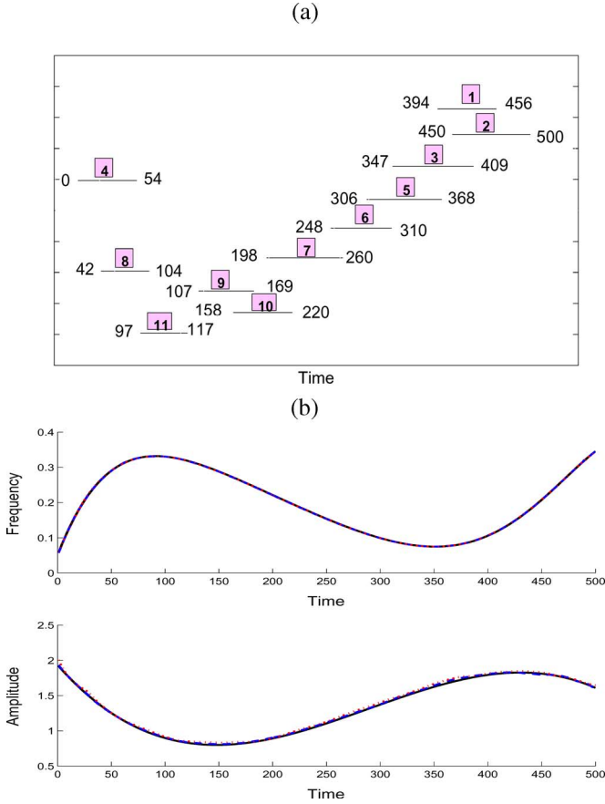
Fig. 3. (a) Nonsequential time segmentation of the signal in Fig. 1. Each segment bears a mention of the starting time, ending time, and processing order (in a box). (b) Estimation of IF (seventh-order polynomial) and IA (cubic polynomial) for the same signal based on the mean of 50 Monte Carlo realizations at a mean SNR equal to 15 dB (—) and 7 dB (···) versus original curves (—).
