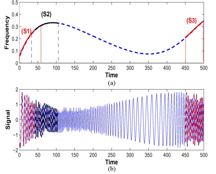
Fig. 1. Examples of short-time segments adapted to a second-order polynomial modeling: (a) IF and (b) the signal. (S1), (S2), and (S3) are three segments of 55, 63, and 51 samples, respectively. The IA and IF are third- and seventh-order polynomials, respectively.
