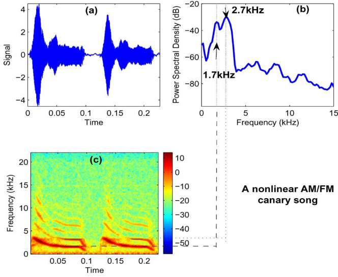
Fig. 12. Canary song: (a) AM/FM signal, (b) power spectral density and (c) spectrogram calculated using a fast Fourier transform of 256 points, a sliding Hanning window of 256-point length, and an overlap of 255.
