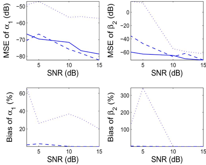
Fig. 6. MSE and bias of the amplitude parameter \alpha_1 and phase parameter \beta_2 (4) of the signal of (23) versus SNRs: ( \cdots ) HAF-based method, ( -- ) the proposed method, and ( — ) the appropriate CRBs.
