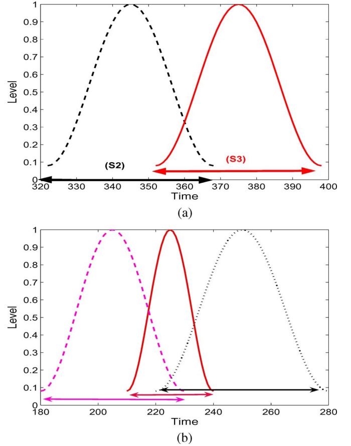
Fig. 2. Merging strategy using Hamming windows for the phase smoothing: Two cases (a) and (b) are possible. (a) Two segments are merged. (b) Three segments are merged.
