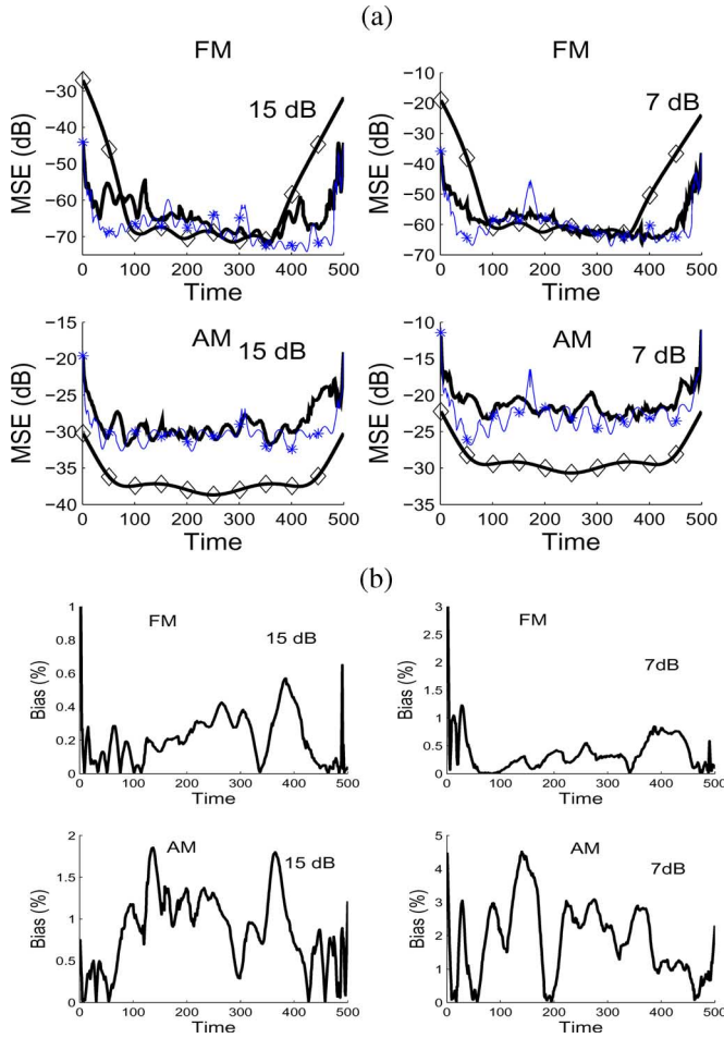
Fig. 8. (a) MSE obtained in the estimation of the frequency and amplitude of the highly nonstationary signal in Fig. 1 using (—) the algorithm proposed, ( \diamond ) the \text{CRB}_P , and ( \ast ) the \text{CRB}_G , at mean SNR = 15 dB (left column) and at 7 dB (right column). The \text{CRB}_P values are calculated at the true orders: the FM is a seventh-order polynomial and the AM is a third polynomial. (b) Biases (—) at mean SNR = 15 dB (left column) and at 7 dB (right column) using the proposed algorithm.
