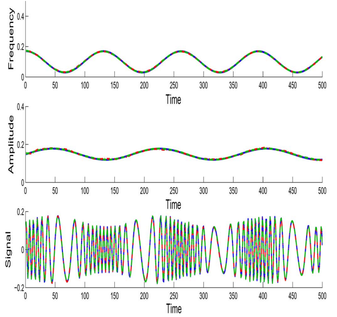
Fig. 10. Original curves of a sinusoidal AM/FM signal (—) and the reconstructed ones: (---) at 15 dB and (- · -) at 7 dB using the proposed algorithm.
