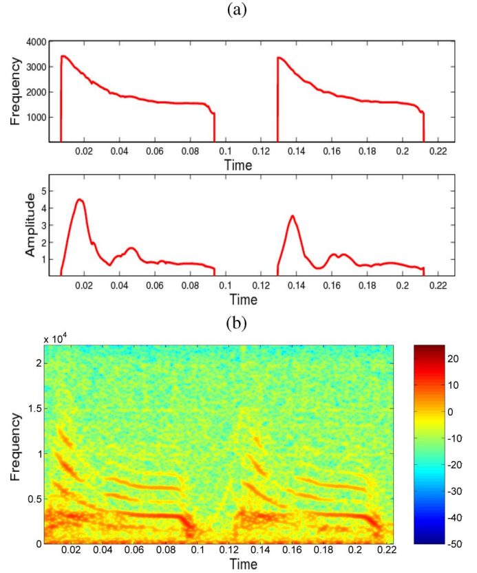
Fig. 13. (a) Estimated FM and AM of the highest energy component of the signal. (b) Spectrogram of the residual signal after removing the highest energy component of the canary song calculated with a fast Fourier transform of 1024 points, a sliding window of 256, and an overlap of 255.
