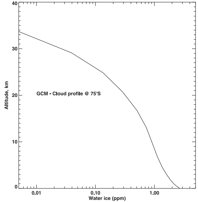
Figure 13. LMD-GCM predictions of the water ice cloud profile at 75°S around northern summer solstice ( L_s 90°). The model predicts an atmospheric water ice content declining continuously throughout the atmosphere, in agreement with SPICAM observations.
