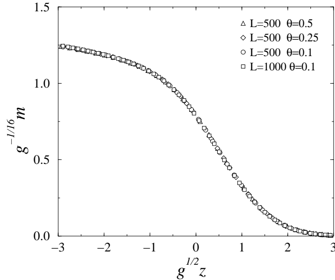
Figure 2. Rescaled magnetization profiles for different chain sizes L and \theta values. The values of the gradient are the same as in figure 1.
